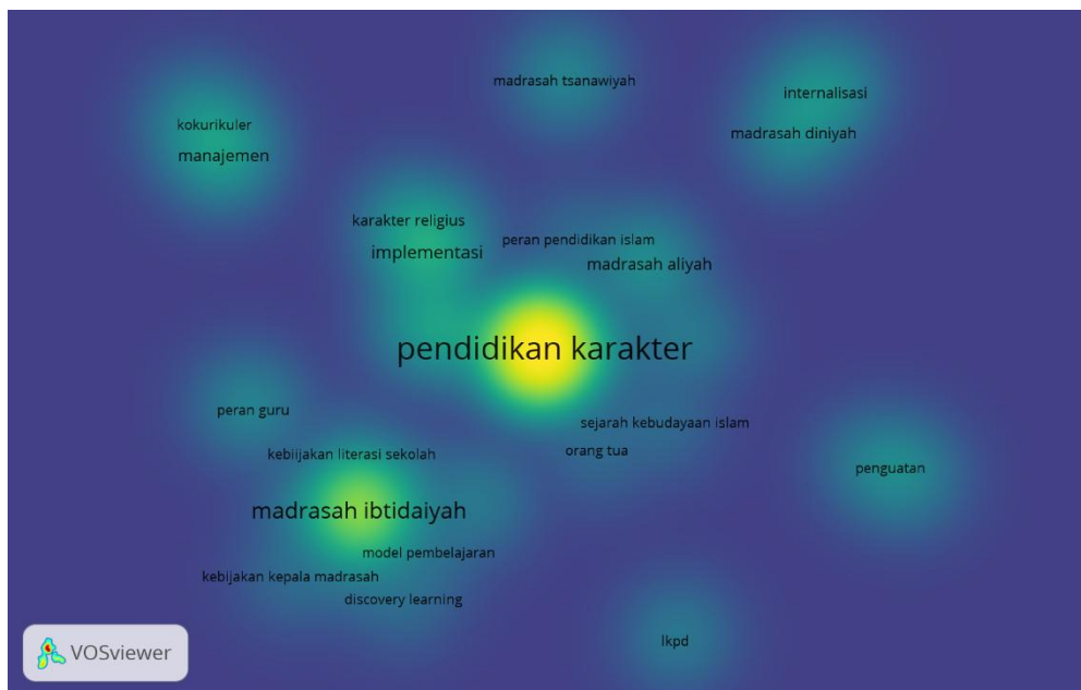
Gambar 5. Density visualization
