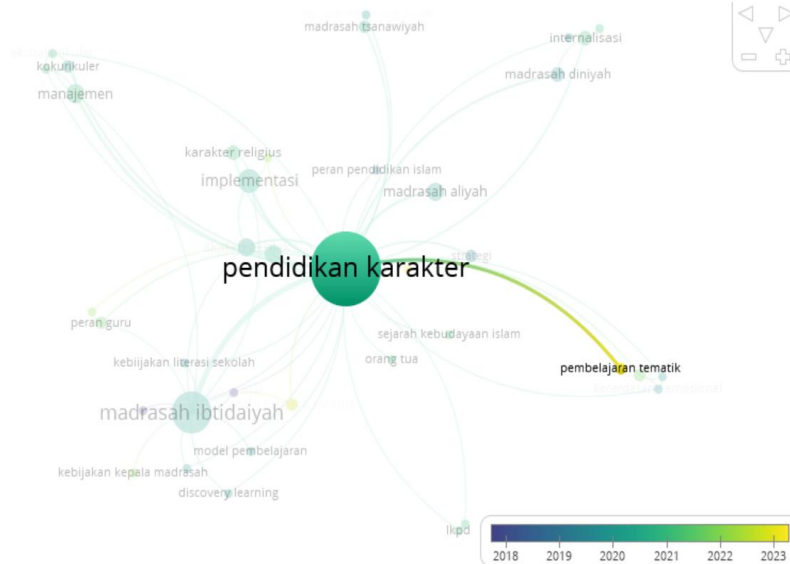
Gambar 4. Overlay visualization
