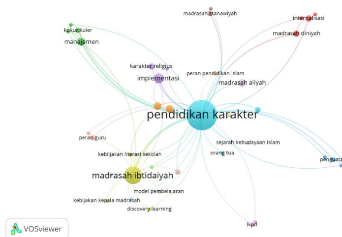
Gambar 3. Network visualization
